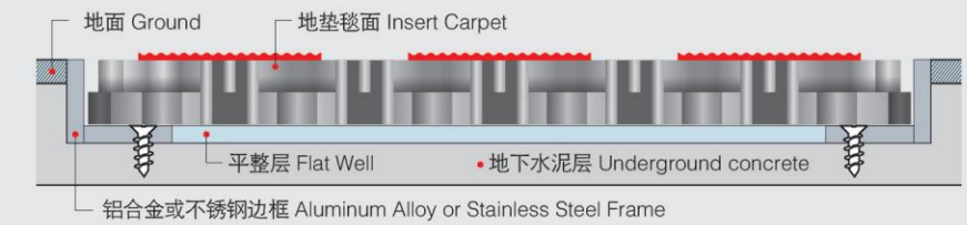
凹槽内铺设 Installation in Groove
